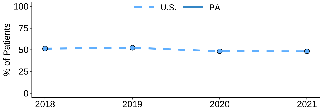
Figure 6: OP-3b Trends in Pennsylvania and All CAHs Nationally
