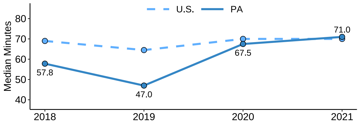
Figure 7: OP-18b Trends in Pennsylvania and All CAHs Nationally
